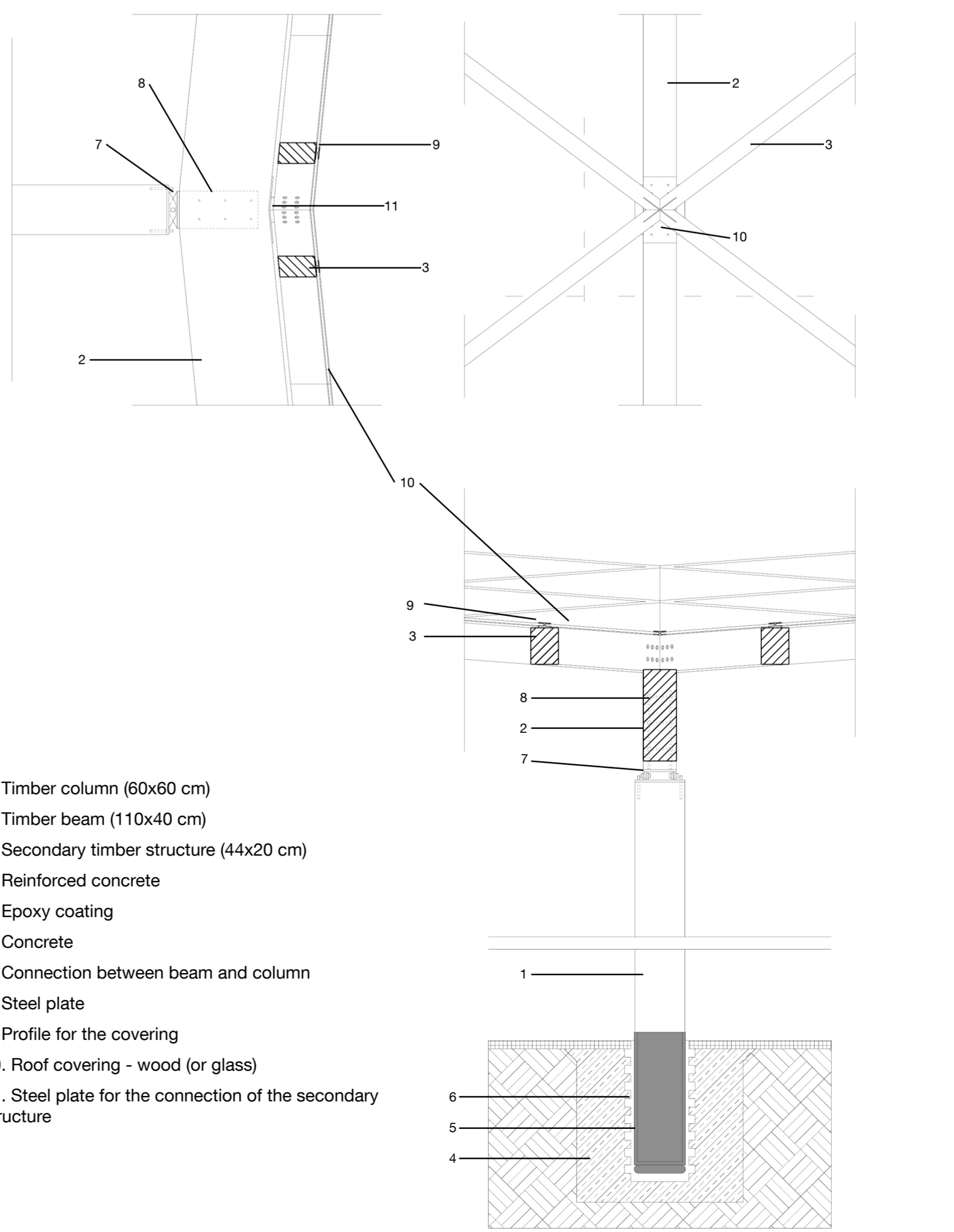
1.50 3 views detail
