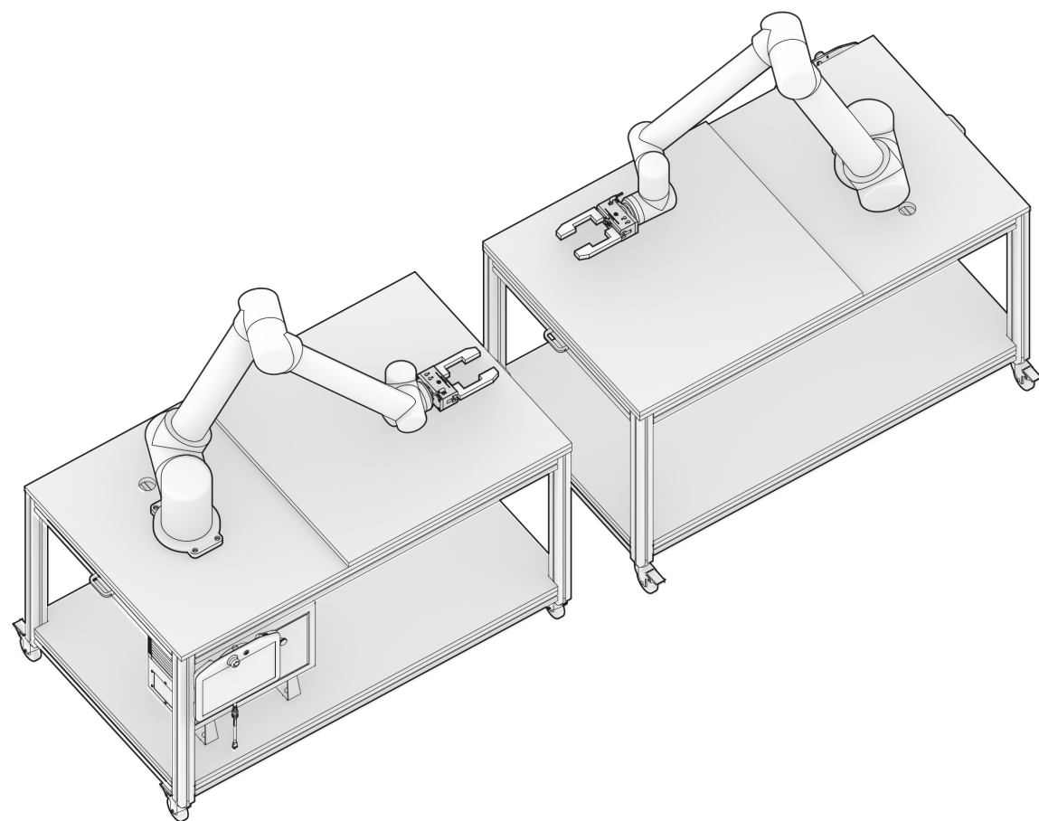
Illustration: Robot setup for the practical experimentation with concepts of robotic fabrication in architecture Image: Augmented Fabrication Lab
